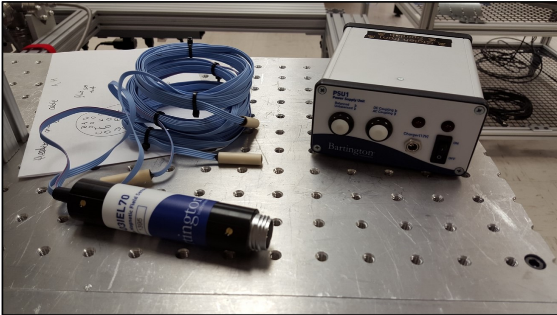
Figure D3: Fluxgate: Bartington Mag03IEL70. 16 kHz excitation frequency, noise floor is 6 \text{ pT}_{\text{rms}}/\sqrt{\text{Hz}} . Power supply: Bartington PSU1. 5 \text{ pT}_{\text{rms}}/\sqrt{\text{Hz}} noise floor. Data acquisition: NI PCie-6320. 16-bit. 2 mV noise floor on 10 V scale.
